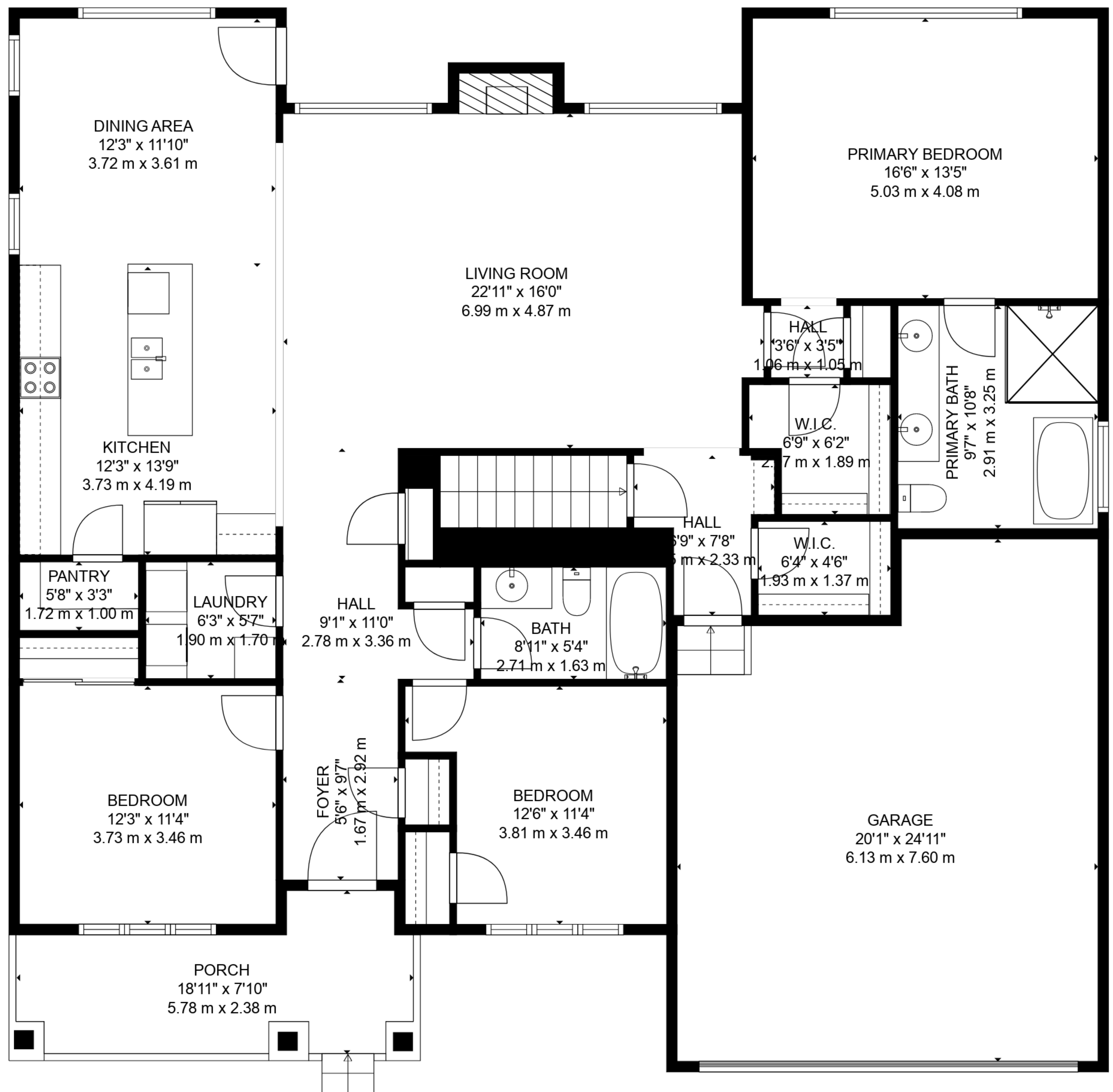
FLOOR 2
