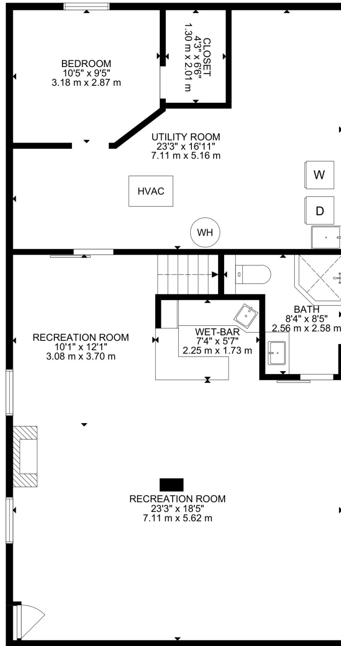
LOWER FLOOR
