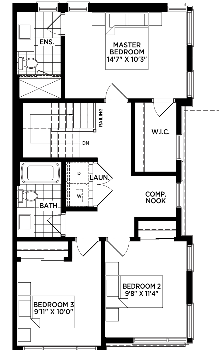
SECOND FLOOR
